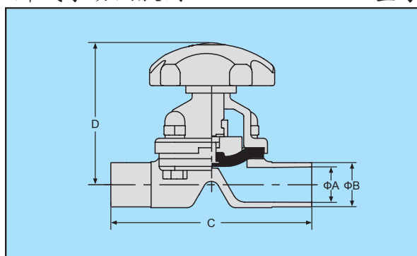
焊式手动隔膜阀
