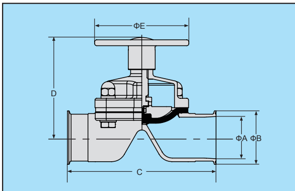
焊式手动隔膜阀
